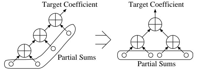
Fig. 1. Tree reduction.
