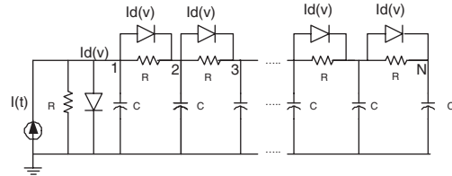
Figure 5: Nonlinear Transmission Line from [16]
