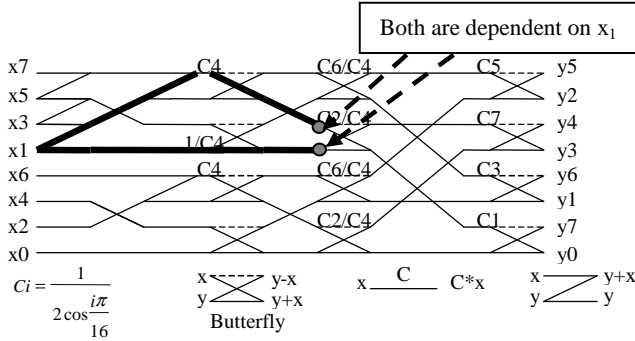
Figure 3: Dataflow of the IDCT algorithm
