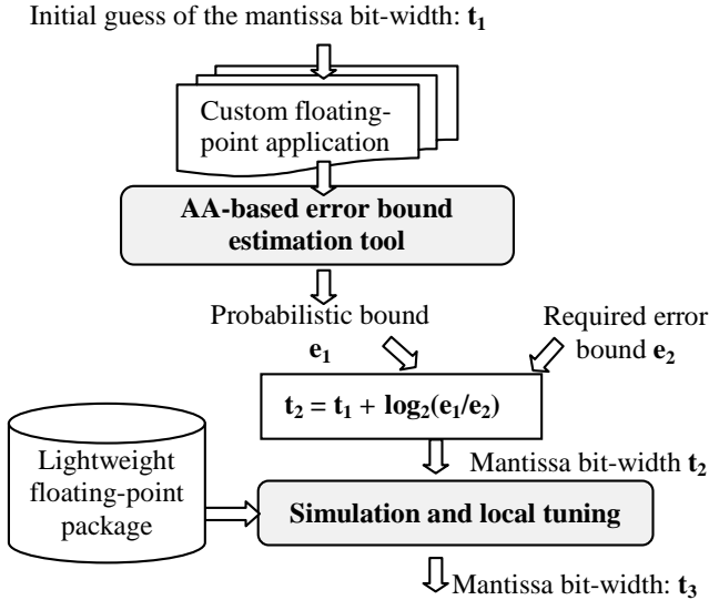
Figure 6: Configuring mantissa bit-width
