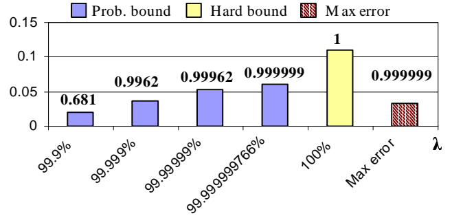
Figure 4: Probabilistic bounds for WHT
