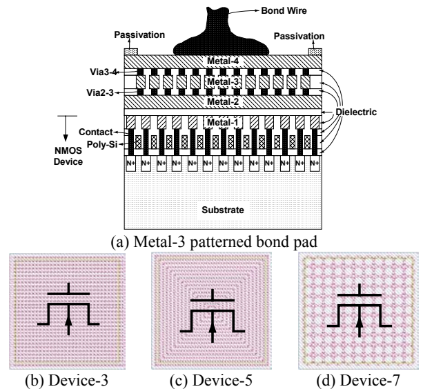
Fig. 3 Layout designs of bond pads with NMOS devices placed under Metal-2. (a) Cross-sectional bond pad structure of Metal-3 patterned devices, (b)-(d) show the patterned Metal-3 layer layouts of Device-3, Device-5, and Device-7, respectively. The NMOS device symbols on the bond pad layout patterns indicate that there is a NMOS transistor under the patterned metal layer(s) for each bond pad.
