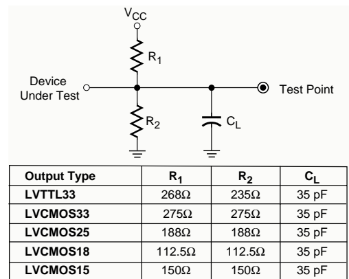
Figure 3: AC Load Circuit
