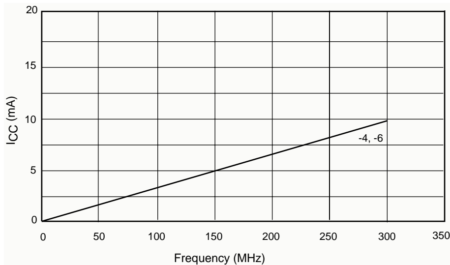
Figure 1: I CC vs Frequency
