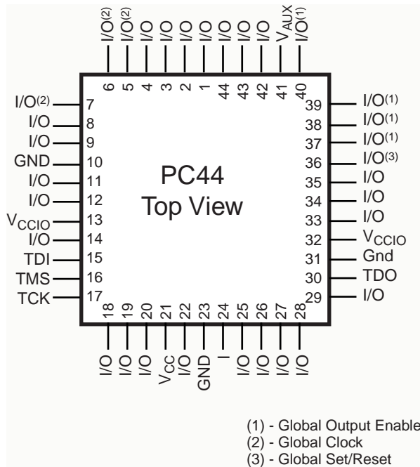
Figure 5: PC44 Package
