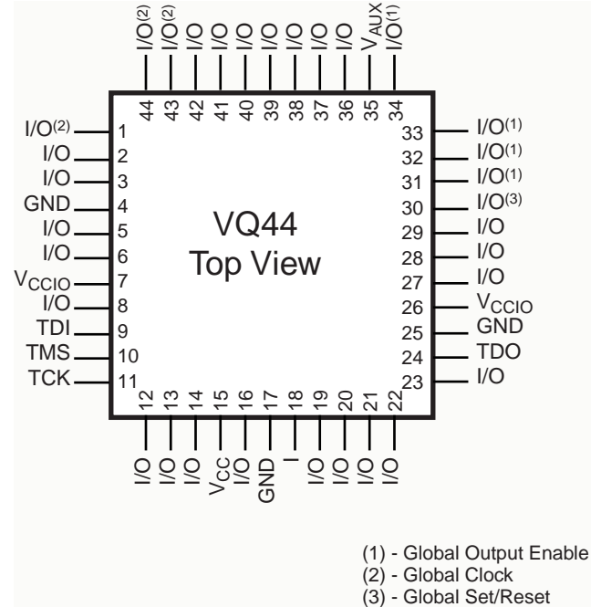
Figure 6: VQ44 Package
