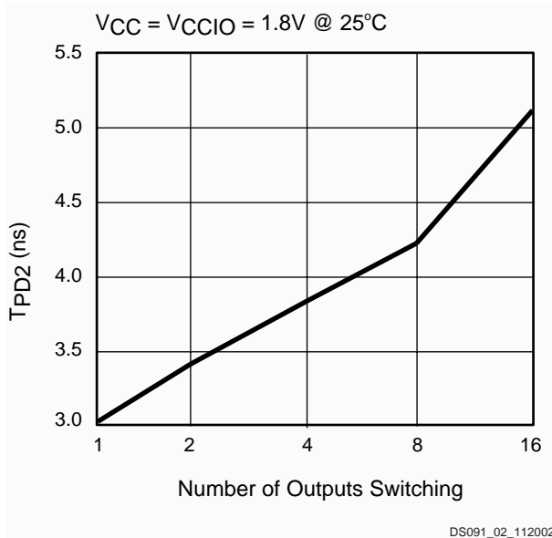
Figure 2: Derating Curve for T PD
