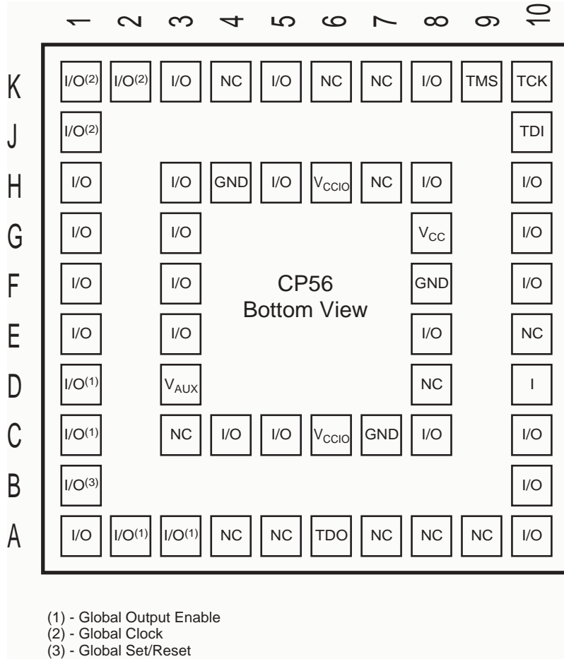
Figure 7: CP56 Package
