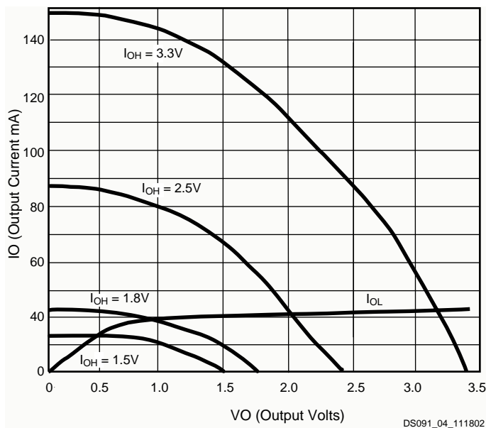
Figure 4: Typical I/V Curve for XC2C32
