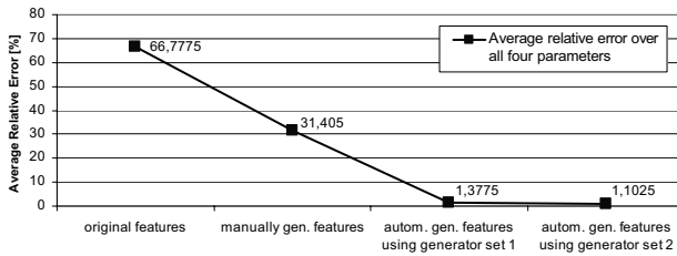
Fig. 1. Average relative error over all four parameters on a two-substance mixture
