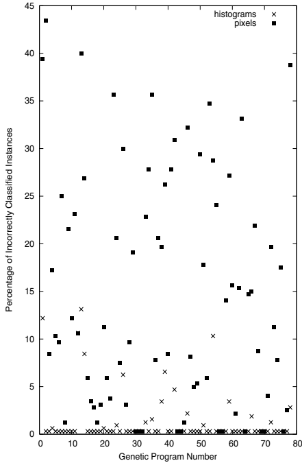
Fig. 4. Error for pixel and histogram approaches
