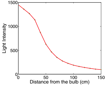
Fig. 2. Distance mapping for the 40w frosted bulb
