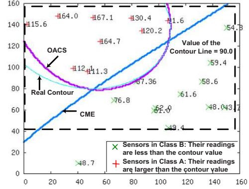
Figure 2. An example of the results generated by CME and OACS
