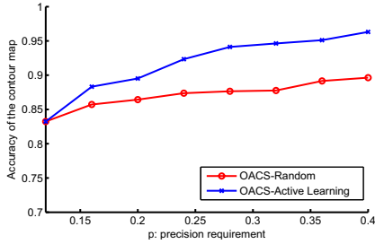
Figure 7. Accuracy as a function of precision requirement: L-enquiry case
