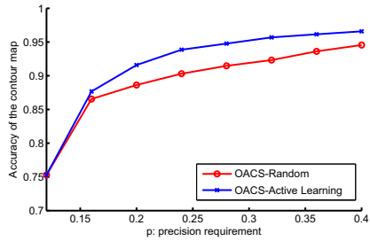
Figure 8. Accuracy as a function of precision requirement: M-enquiry case
