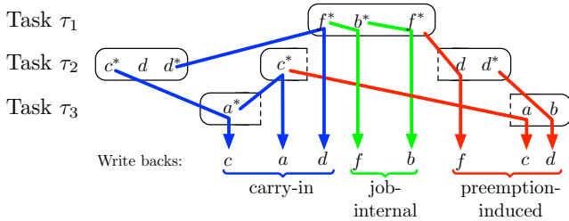
Figure 1: Example illustrating different kinds of write backs.
