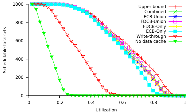
Figure 5: Number of schedulable task sets (FPNS).
