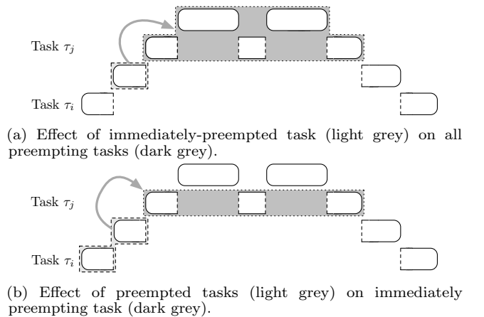
Figure 3: Methods of accounting for lp-carry-in write backs.
