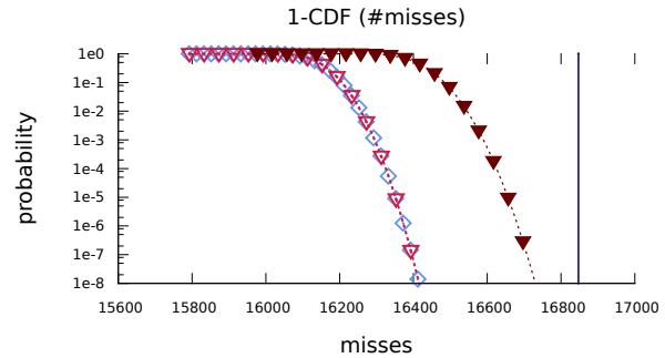
Fig. 12. Analysis results for fft, 141 distinct blocks, 18Ka.
