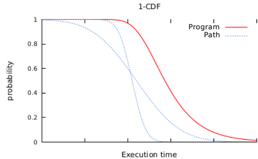
Fig. 1. Relation between paths and program pWCET.
