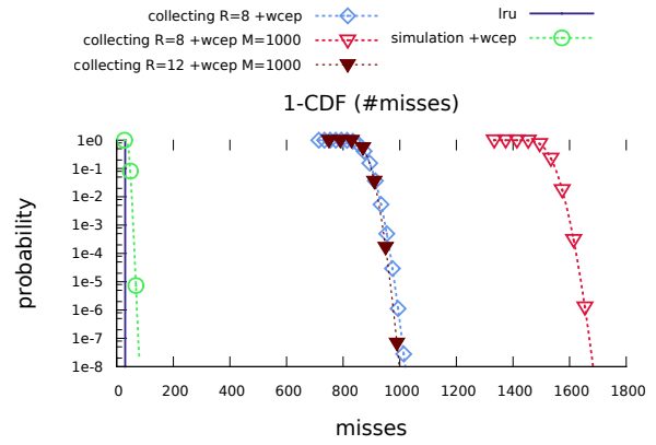
Fig. 10. Analysis results for matmult, 28 distinct blocks, 63Ka.
