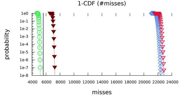
Fig. 11. Analysis results for edn, 166 distinct blocks, 67Ka.
