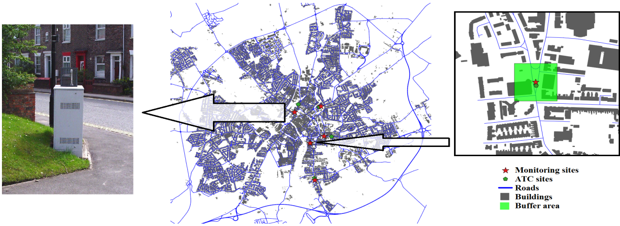
Fig. 1. Heworth monitoring station (left), map of the modelling area (centre), Buffer area for the Fishergate monitoring station (right)
