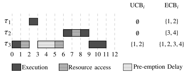
Fig. 6. Tasks \tau_2 and \tau_3 share a common resource x , \tau_3 starts to execute, blocks \tau_2 , which is released at time 1, and is pre-empted by \tau_1 . Thus, the finishing time of \tau_2 is delayed not only by the time for which \tau_3 accesses the resource, but also by the additional pre-emption delay, reloading UCBs \{1, 2\} after the pre-emption of the resource access of task \tau_3 by task \tau_1 .
