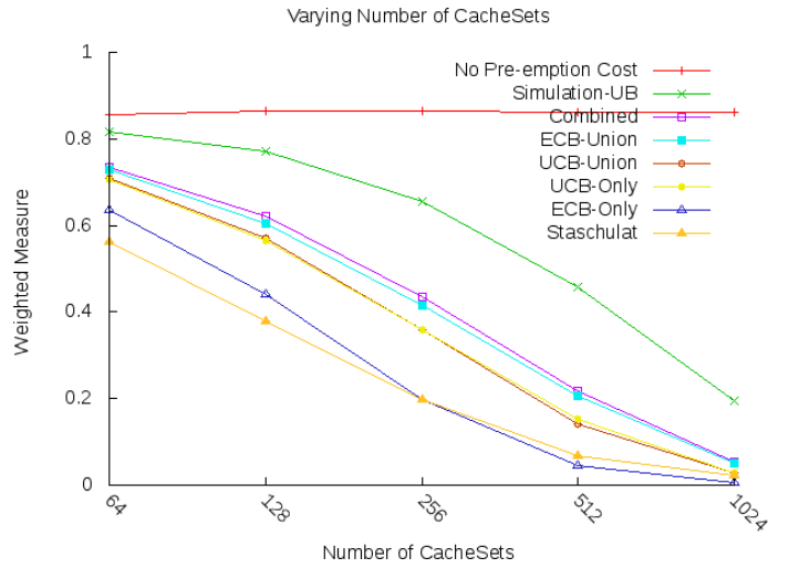
Fig. 11. Weighted schedulability measure; varying number of cache sets from 2^5 = 64 to 2^{10} = 1024
