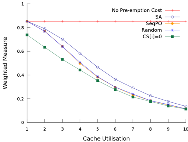
Figure 9. Varying the cache utilisation from 1 to 10
