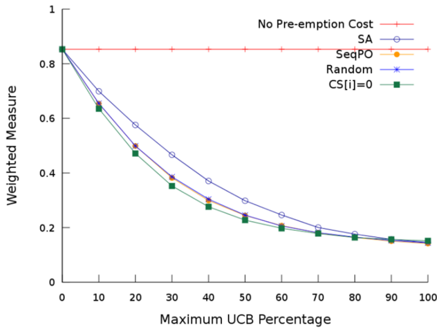
Figure 8. Varying the maximum UCB percentage from 0% to 100%
