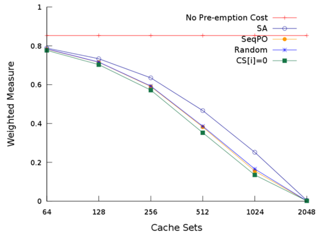
Figure 10. Varying the number of cache sets from 64 to 2048
