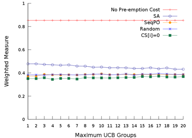
Figure 7. Varying the number of maximum number of UCB groups from 1 to 20
